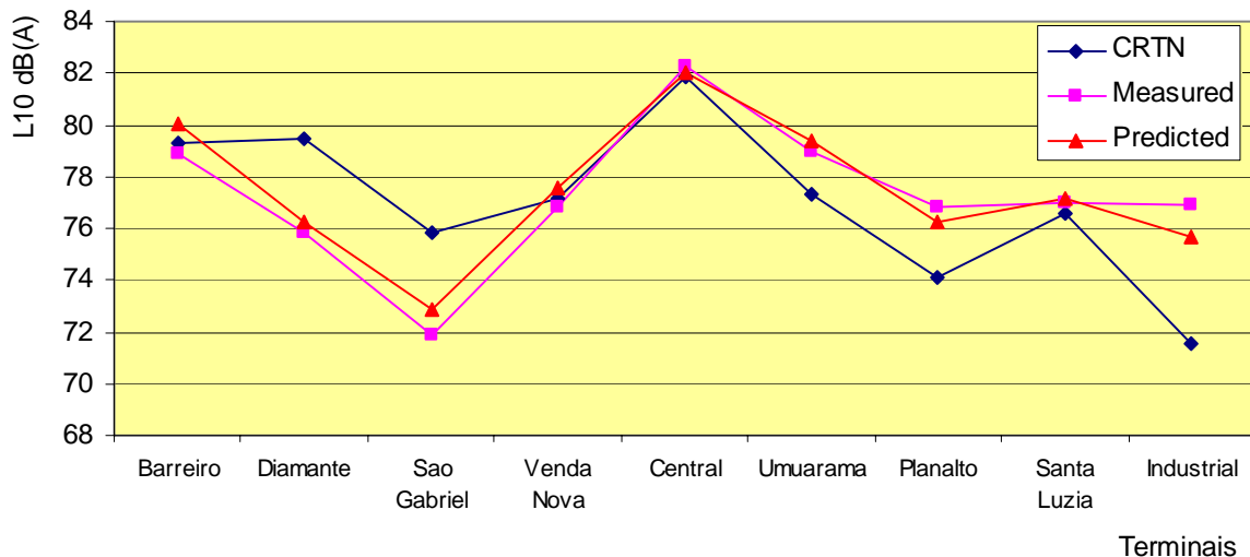
Figure 1 – L_{10} Values obtained using the CRTN method, field measurements and the statistical model developed.
