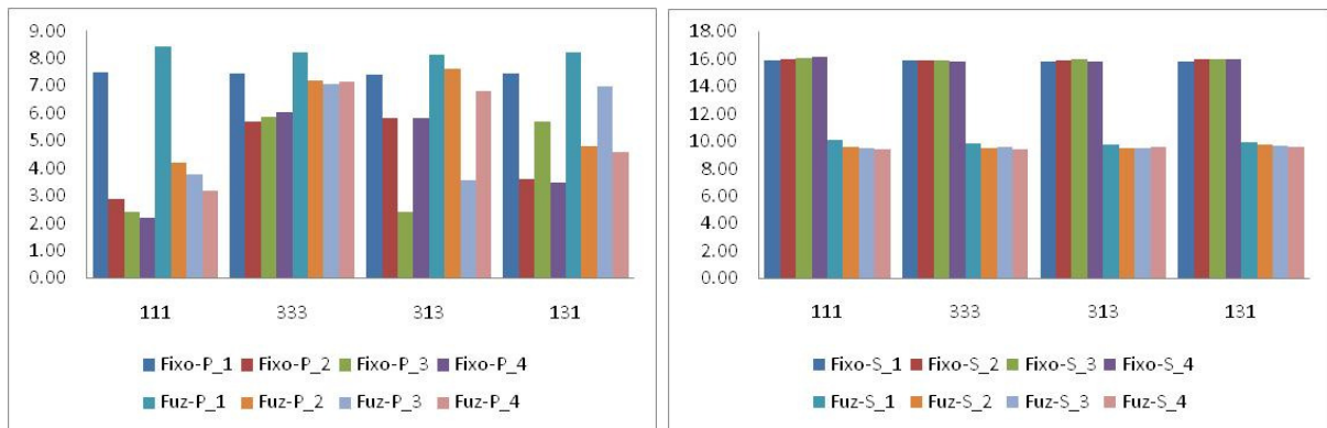
(a) Arterial road (b) Secondary roads Figure 13 Average delay per intersection approach for low volume under the two control modes studied: Fuzzy (Fuz) and Fixed-time coordinated (Fix)
