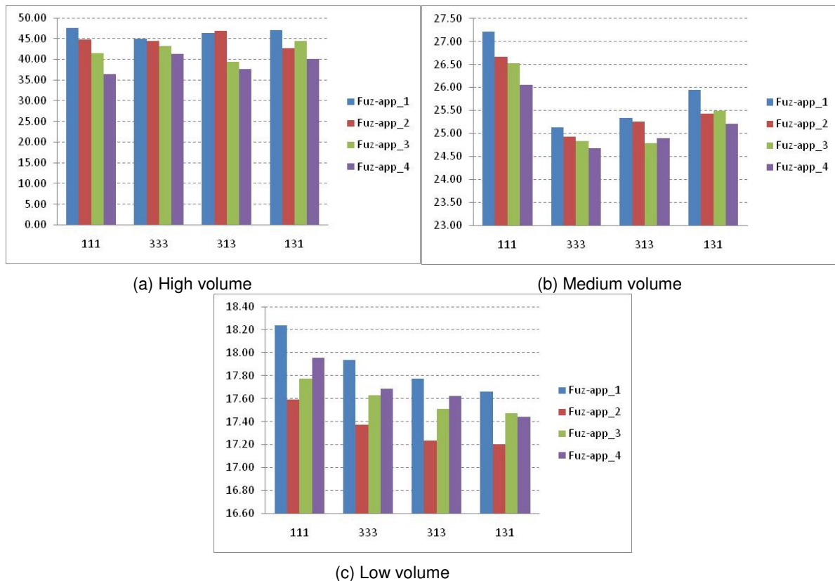
(a) High volume (b) Medium volume (c) Low volume Figure 9 Average green time for the arterial road approach of each intersection
