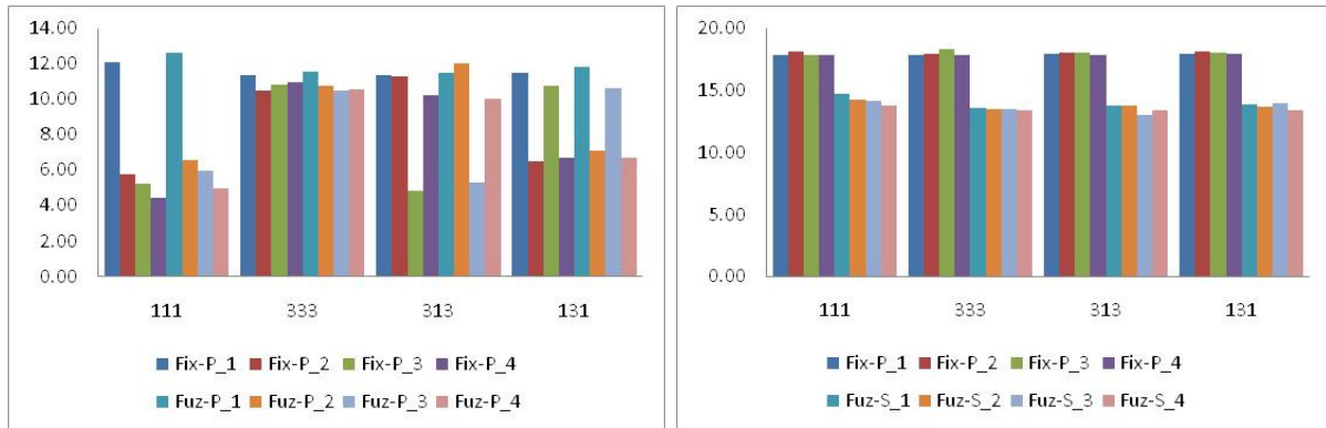
(a) Arterial road (b) Secondary roads Figure 12 Average delay per intersection approach for medium volume under the two control modes studied: Fuzzy (Fuz) and Fixed-time coordinated (Fix)
